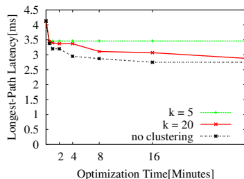
Figure 9: MIP Convergence with k-means: Longest Path
