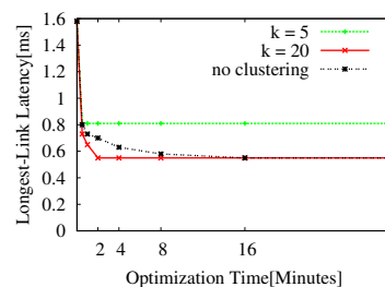
Figure 6: CP Convergence with k-means: Longest Link
