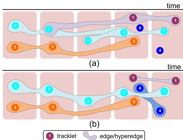
Figure 1: (a) Two previous methods using 3-uniform hypergraph H^2T (Wen et al. 2014) and FH^2T (Wen et al. 2016), often fails to describe the dependencies among tracklets, when occlusion or missed detection happen. (b) The proposed method uses the non-uniform hypergraph to encode different degrees of dependencies among tracklets effectively.
