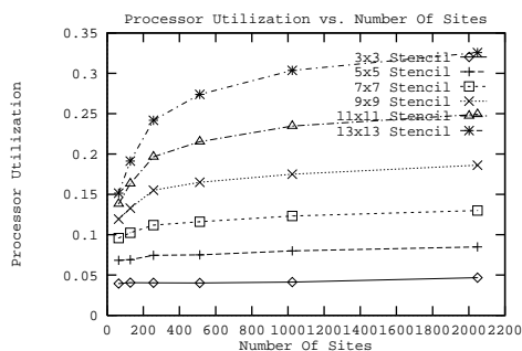
Figure 2: Processor Utilization of MasPar MP-1
