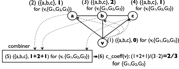
Fig. 15 Clustering Coefficient Example
