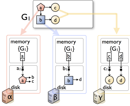
(a) Initial creation of graph G_1 at time 1, when each vertex and its edges are assigned to a server. In this example, servers \alpha and \beta are unchanged at times 2 and 3.
