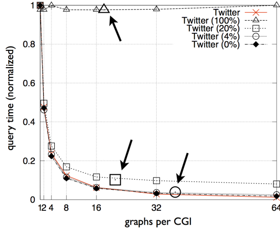
Fig. 24 Query Time: Average Degree
