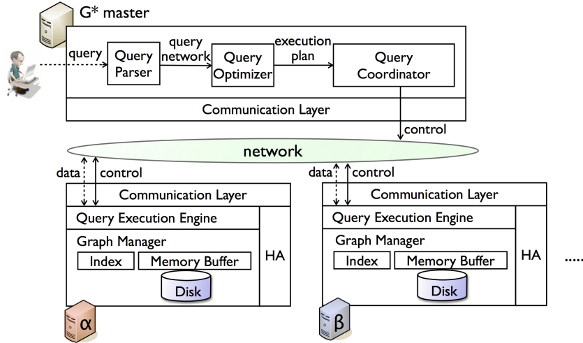
Fig. 1 G^* Architecture
