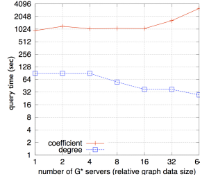
Fig. 27 Yahoo! scale up
