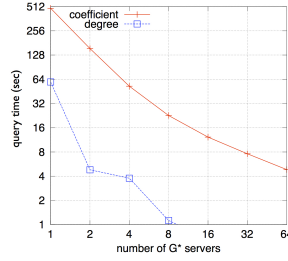
Fig. 30 Yahoo! speed up
