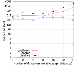
Fig. 28 Tree scale up
