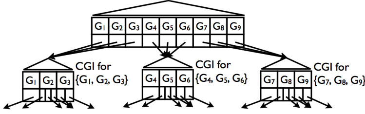
Fig. 10 CGI Splitting Example
