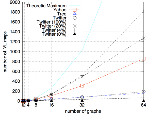
Fig. 22 Number of VL Maps
