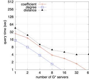
Fig. 31 Tree speed up
