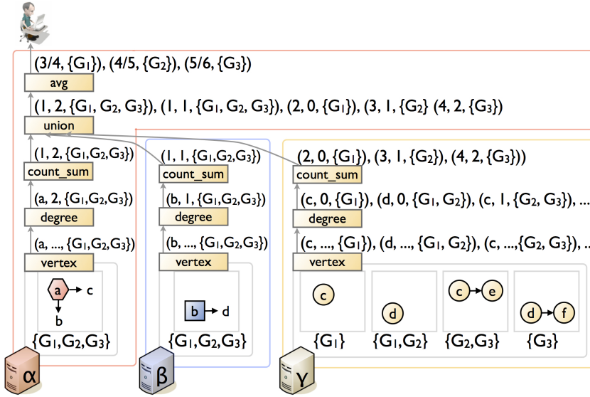
Fig. 3 Distributed Computation of Average Degree
