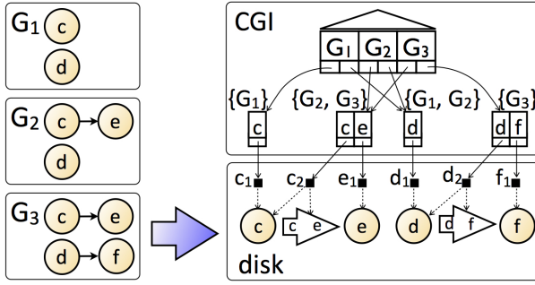
(b) Server \gamma at time 3. Vertex e and edge (c, e) having been added in graph G_2 at time 2, server \gamma now stores two versions of c ( c_1 in G_1 and c_2 with an edge to e in G_2 ) in a deduplicated manner. Now at time 3, with the addition of vertex f and edge (d, f) in graph G_3 , server \gamma stores two versions of d ( d_1 in both G_1 and G_2 , and d_2 with an edge to f in G_3 ).
