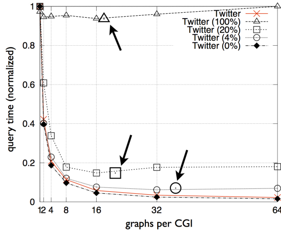
Fig. 25 Query Time: Clustering Coefficient
