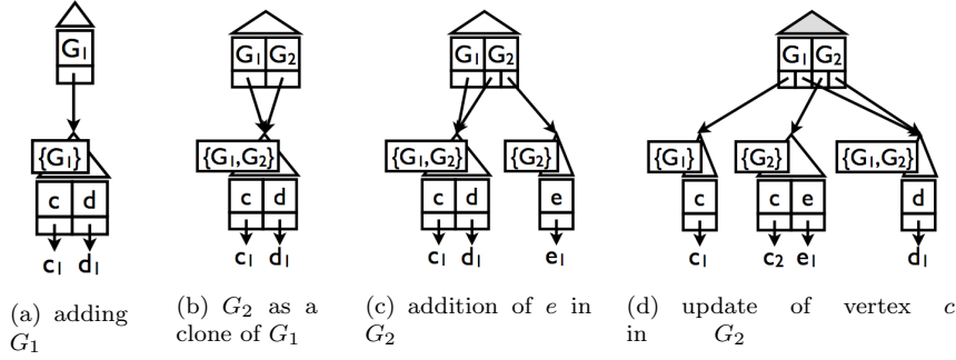
Fig. 7 CGI Update Examples. Figures 7(a) and 7(d) show server \gamma 's CGI in Figures 5(a) and 5(b), respectively.
