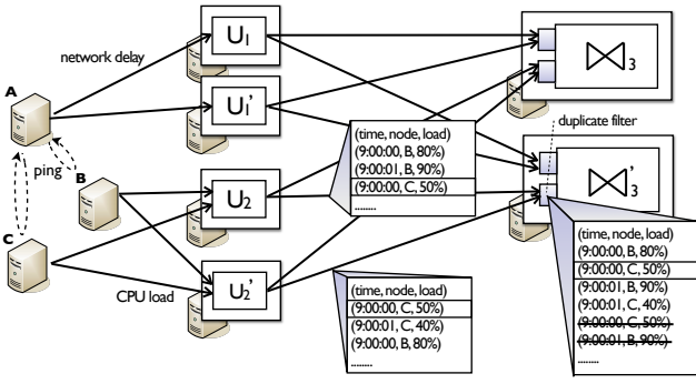
Figure 1: Replication Model. Nodes B and C report their CPU usage to replicas U_2 and U_2' . These replicas merge streams and send the result to D_3 in parallel. D_3 uses whichever tuple arrives first from U_2 and U_2' , while ignoring duplicates (see those struck-through).
