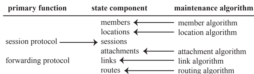
Figure 4: Major components of a layer. Arrows show which protocol or algorithm writes a state component.
