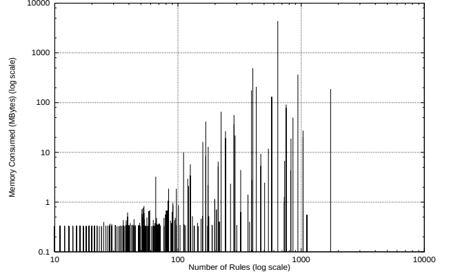
Figure 10: The RFC storage requirements in Megabytes for two Phases using the classifiers available to us. This special case of RFC is identical to the Crossproducting method of [17].
