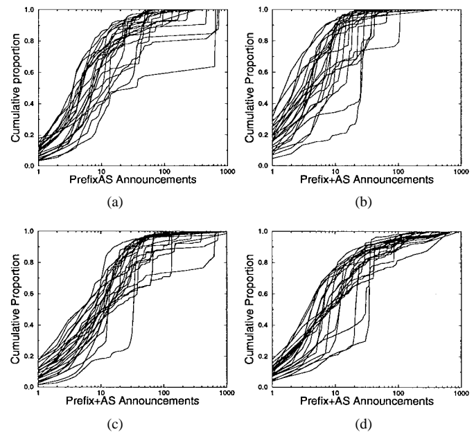
Fig. 7. Cumulative distribution of prefix + AS routing updates measured at the Mae-East exchange point during August 1996. (a) AADiff. (b) WADiff. (c) AADup. (d) WADup. Each line represents a different day in August. A single line shows that day's cumulative distribution function. The function's independent parameter is shown on the horizontal axis, which denotes the number of prefix + AS pairs that generated the corresponding difference in the cumulative output. For example, a point (10, 0.6) on a line denotes that 60% of that day's update events are represented by the set of routes (given as prefix + AS pairs) that exhibited that event ten times or less on that day.
