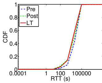
Figure 4.2: RTT.
