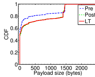
Figure 4.3: Payload size.
