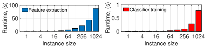
Fig. 23: SYMMeTRy runtime for feature extraction (left) and classifier training (right). Both feature extraction and classifier training time grow exponentially with the instance size.
