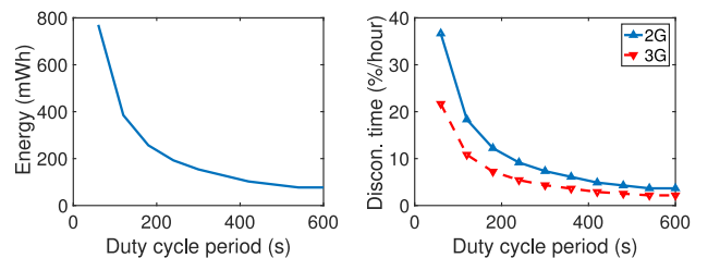
(a) Power consumption increases exponentially as P increases.
